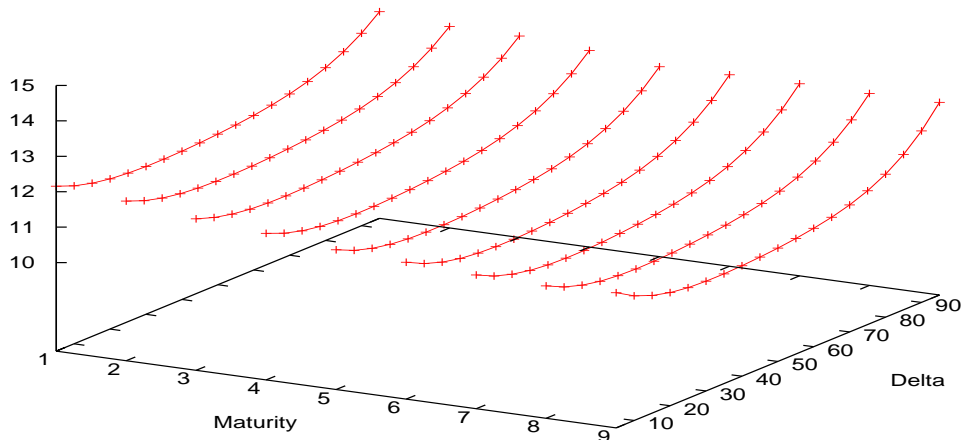
Figure 1: EUR/USD implied volatilities (in percentage points) as of 12 February 2004.
