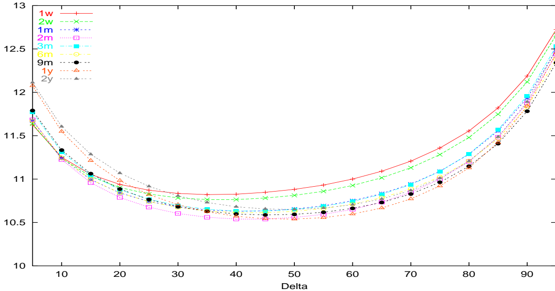
Figure 3: The three-month implied volatility smiles starting at different forward times.
