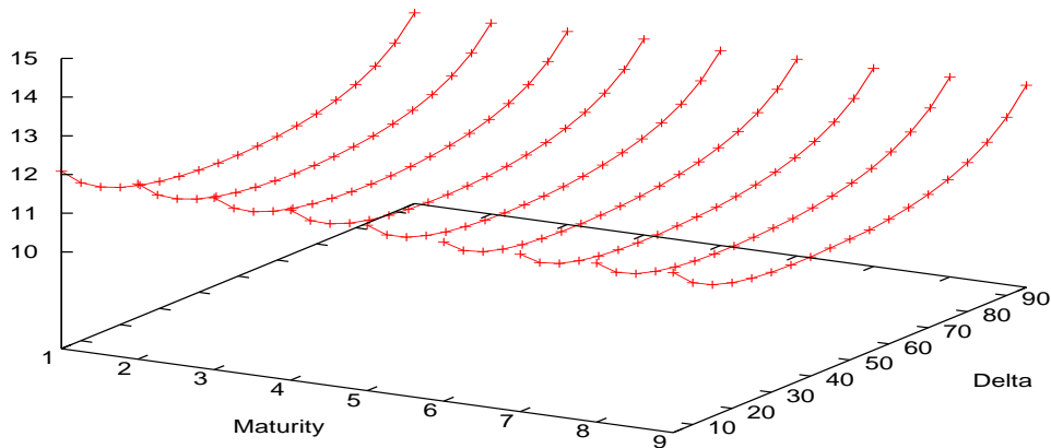
Figure 2: The three-month forward volatility surface.
